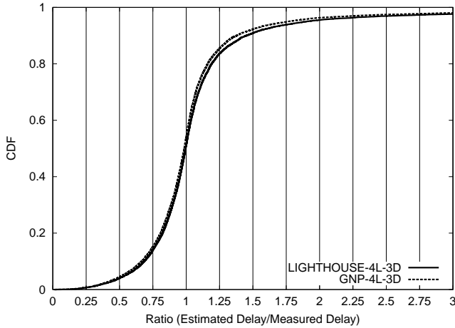
Figure 6: Accuracy of Lighthouse: Extrapolation
