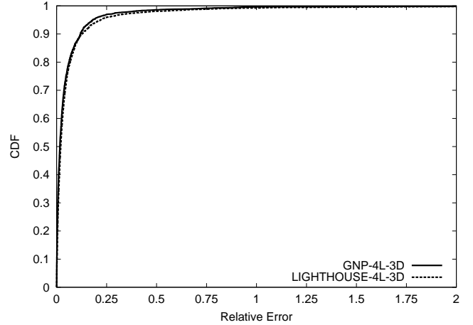
Figure 5: Accuracy of Lighthouse: Calibration
