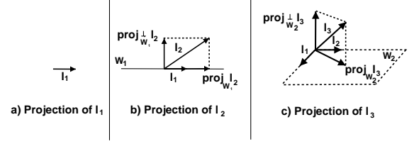
Figure 4: Gram-Schmidt Process
